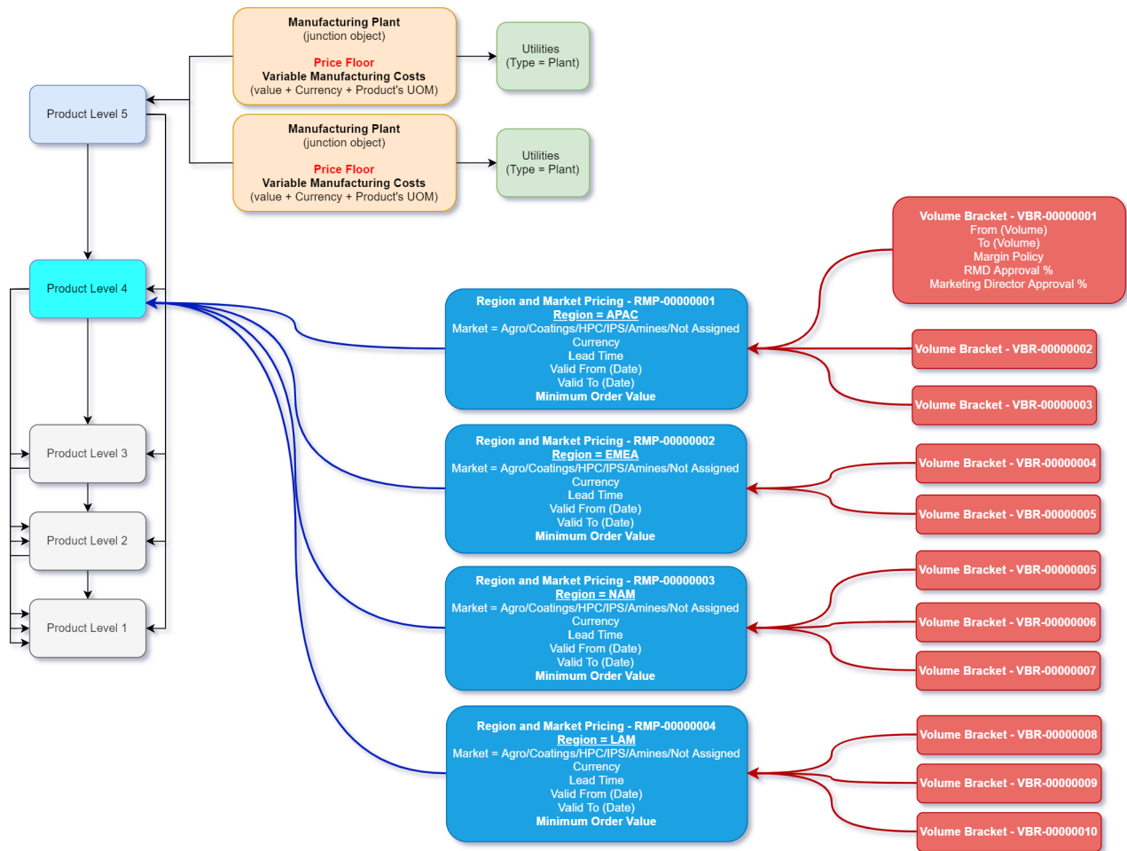
Current Data Model ERD (June 2022)
