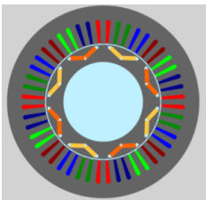
Motor Performance Simulation
