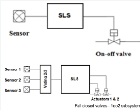
Instrumented safeguards
