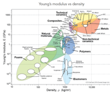
Metal / Polymer generic comparative properties
