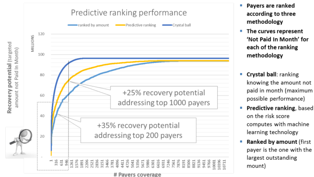
Figure 10. Ranking performance
