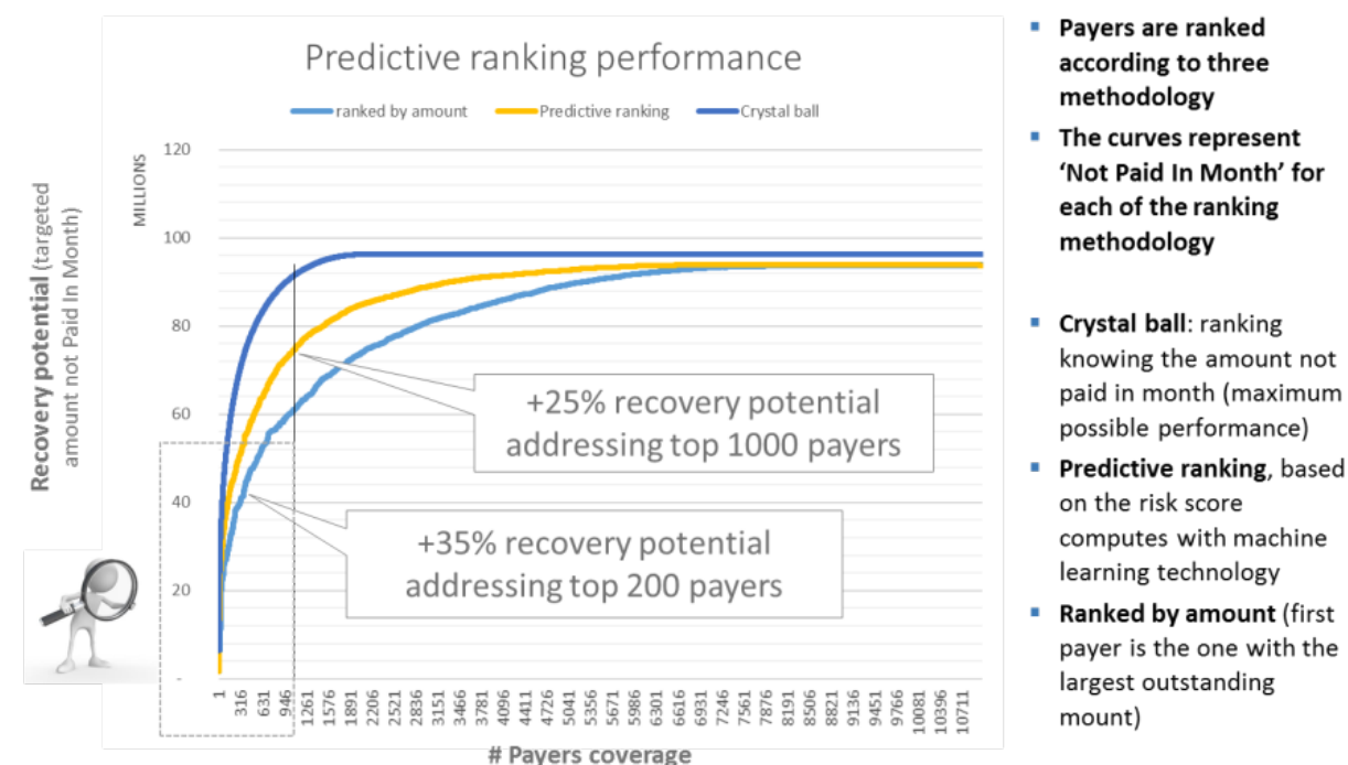
Figure 10. Ranking performance
