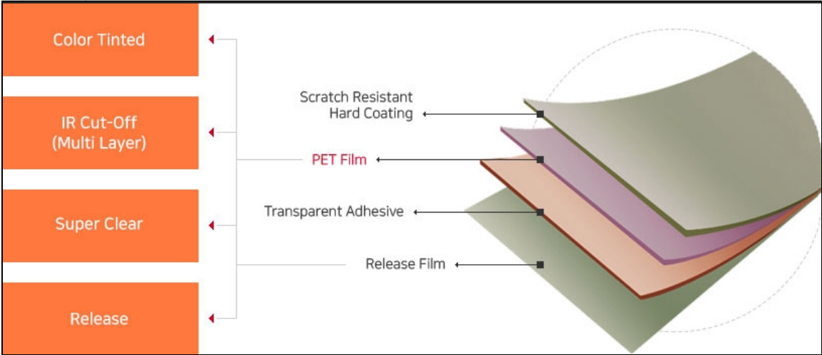
Ex.) Window protection film structure
