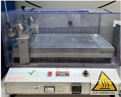
Stendifilm Elcometer (25-100 °C; speed 5-100 mm/s)
