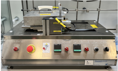
Film Applicator DeltaE (25-300 °C; speed 5-100 mm/s)
