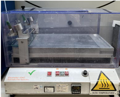
Stendifilm Elcometer (25-100 °C; speed 5-100 mm/s)
