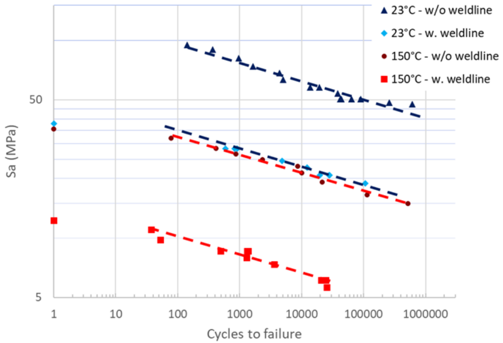
Fatigue Behavior of IXEF 1022 - Effect of Weldline 0deg coupons ; R=0.1
