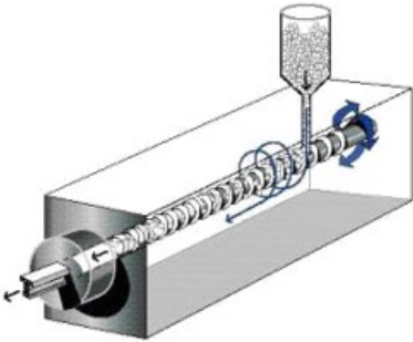
Extrusion Theory
