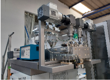
Reactive Extrusion
